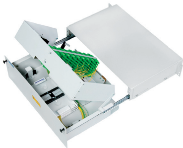
BPK-19 19" Distribution Panel
