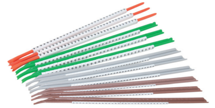
OZNL Cable Markers on Stick Dispenser
